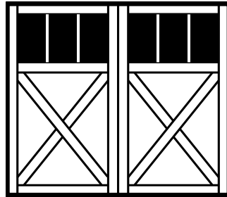
Cross-buck Panel
